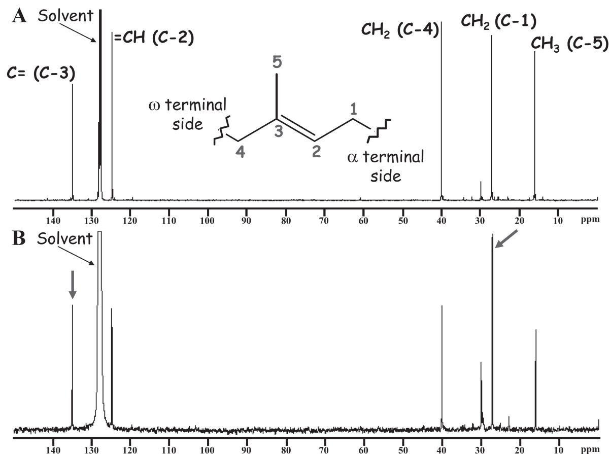
Fig. 8. ^{13}\text{C} NMR spectra of EU-rubber in the feeding experiment with [2-^{13}\text{C}] sodium pyruvate (B) and control (A). The signals pointed by arrows [(C-1) and (C-3)] increased compared to those of the other positions. [2-^{13}\text{C}] Sodium pyruvate was incorporated as an intermediate of both mevalonate and MEP pathways in this feeding experiment (see Fig. 7).
